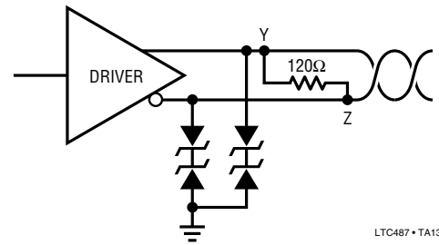
Figure 12. ESD Protection with TransZorbs
