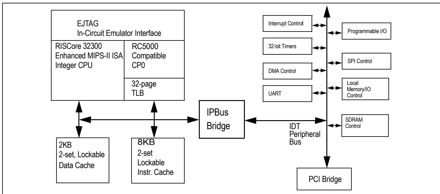
Figure 1 RC32332 Block Diagram
