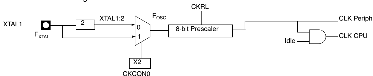
Figure 6-1. Clock Generation Diagram
