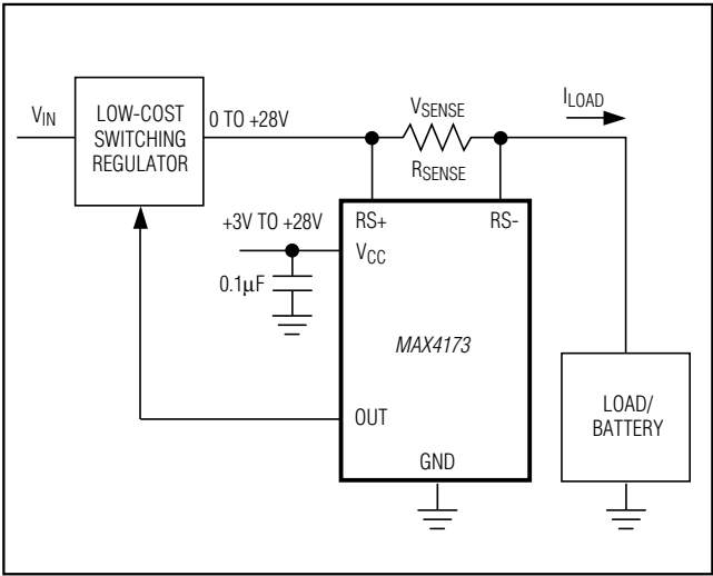
Figure 3. Current Source
