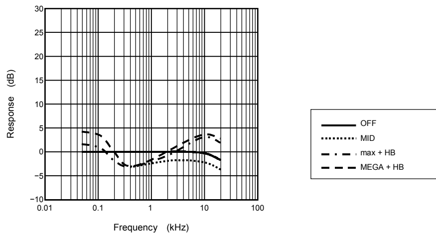
c) V_{in} = 0\text{dB} input, DBB OFF, 1 kHz = 0dB.
