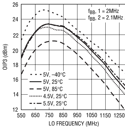
Output IP3 vs LO Frequency
