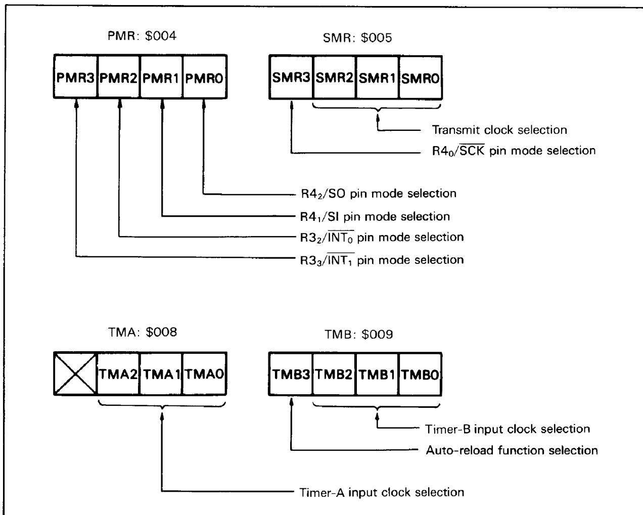
Figure 14 Mode Register Configuration and Function
