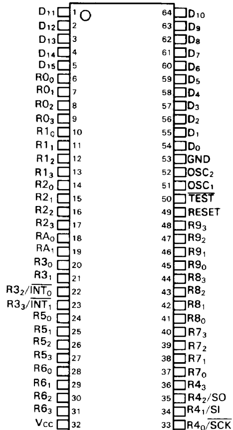
(DP-64S,DC-64S)
