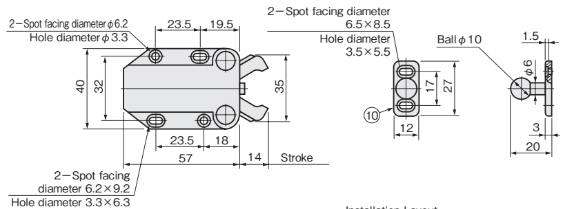
Installation Layout
