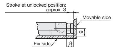
Installation Layout
