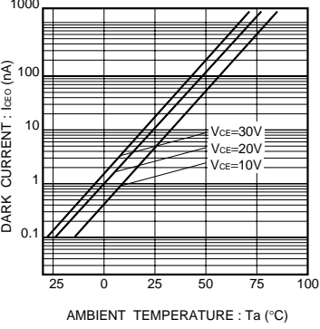
Fig.9 Dark current vs. ambient temperature
