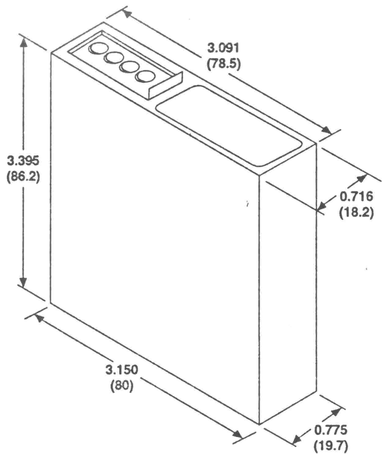
Figure 5. Outline Dimensions
