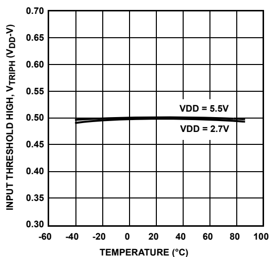
FIGURE 5. V_{TRIP\_H} VOLTAGE
