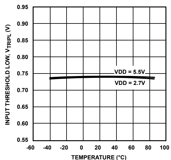
FIGURE 4. V_{TRIPL} VOLTAGE
