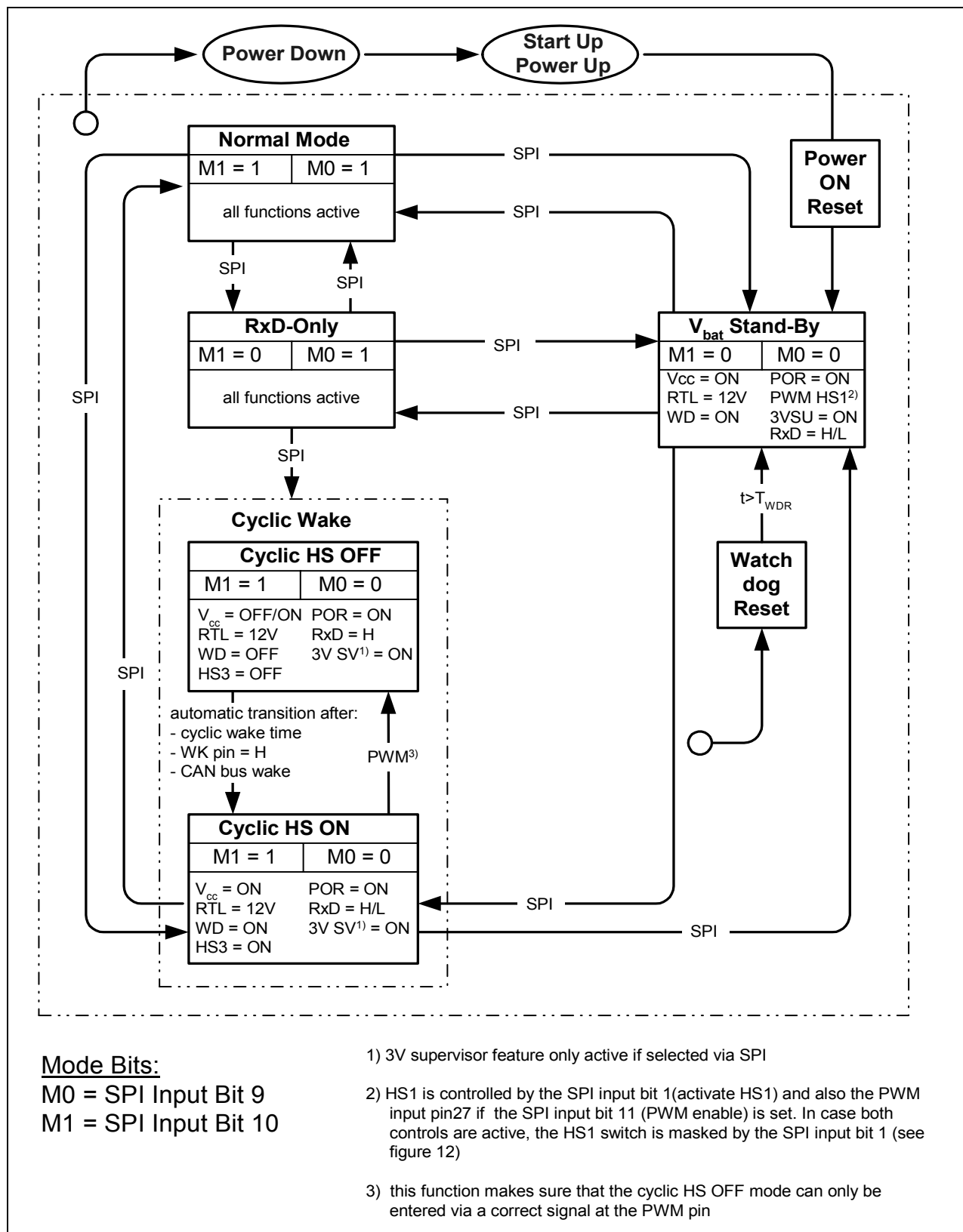
Figure 3 State Diagram
