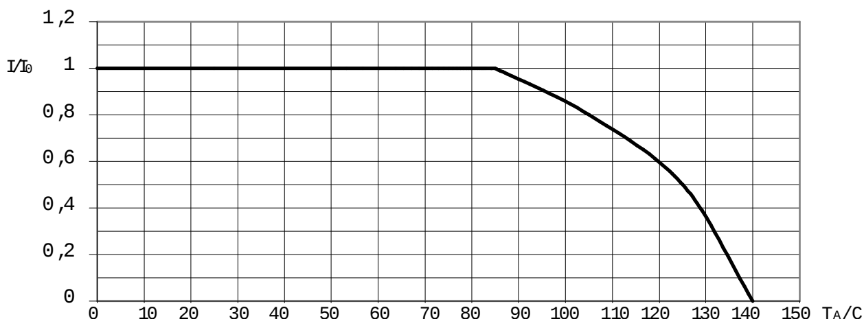
B82464-XXXX-X: current derating versus ambient temperature
