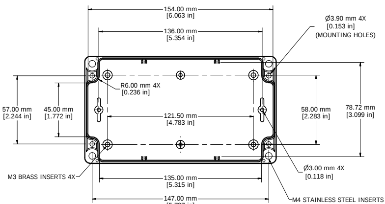
BOX - INSIDE
