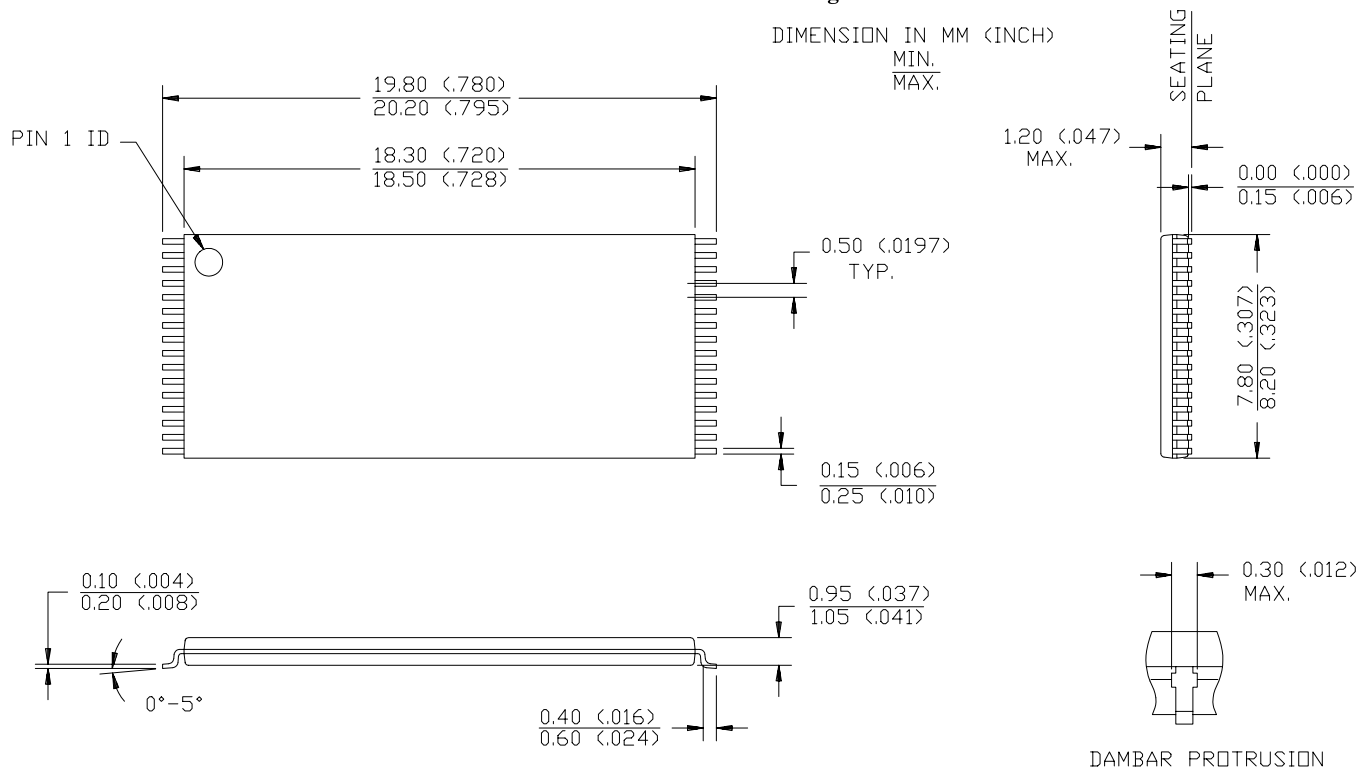
32-Lead Thin Small Outline Package Z32
