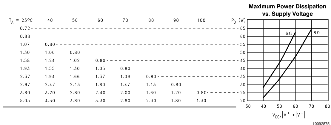
Max Heatsink Thermal Resistance ( ^{\circ}\text{C}/\text{W} ) at the Specified Ambient Temperature ( ^{\circ}\text{C} )
