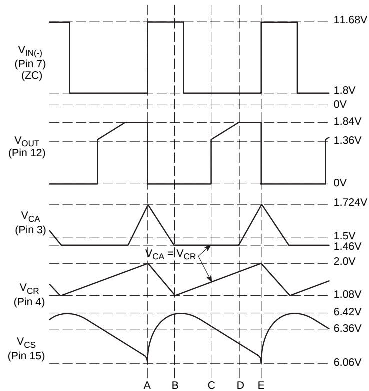
Figure 17. Run Mode 2000 RPM (Frequency: 66.67 Hz @ 5.0 ms)
