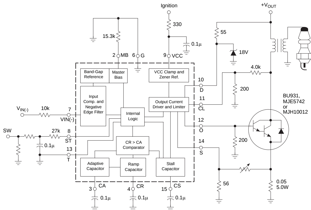
Figure 13. Typical Ignition Circuit Application
