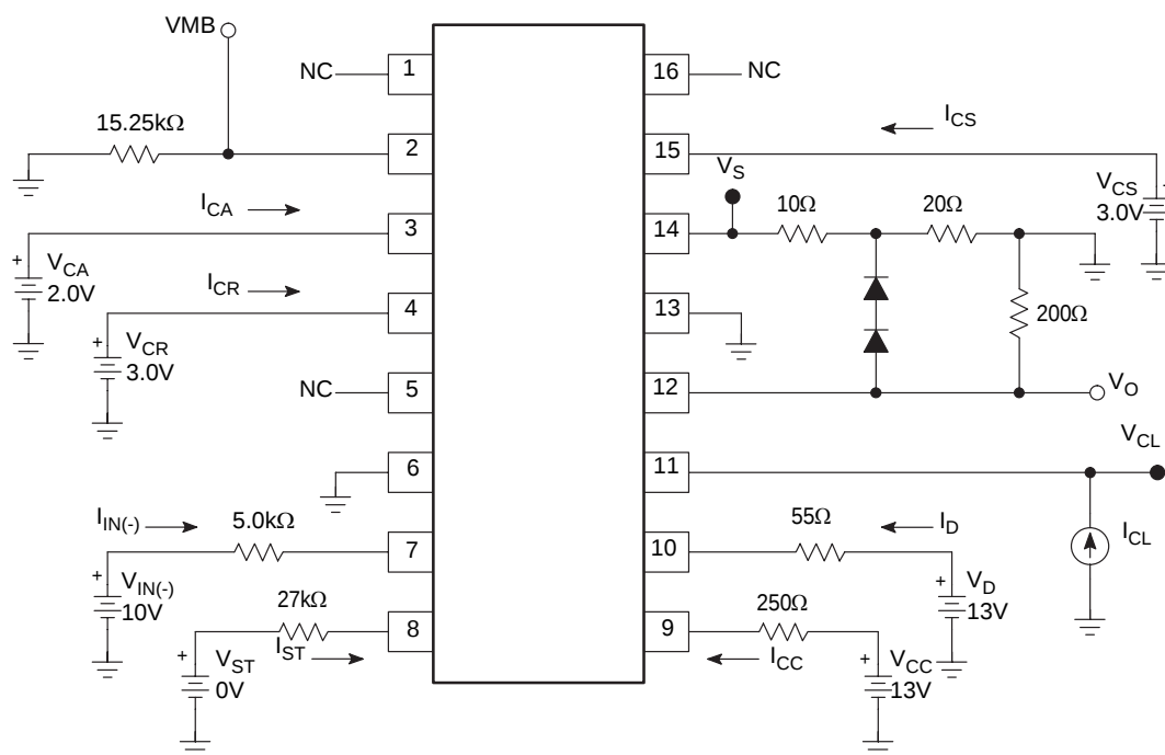
Figure 4. Test Circuit
