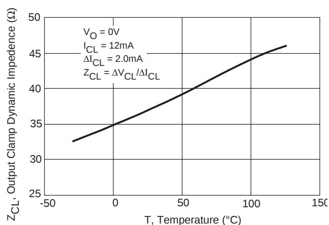
Figure 11. Output Clamp Dynamic Impedance versus Temperature
