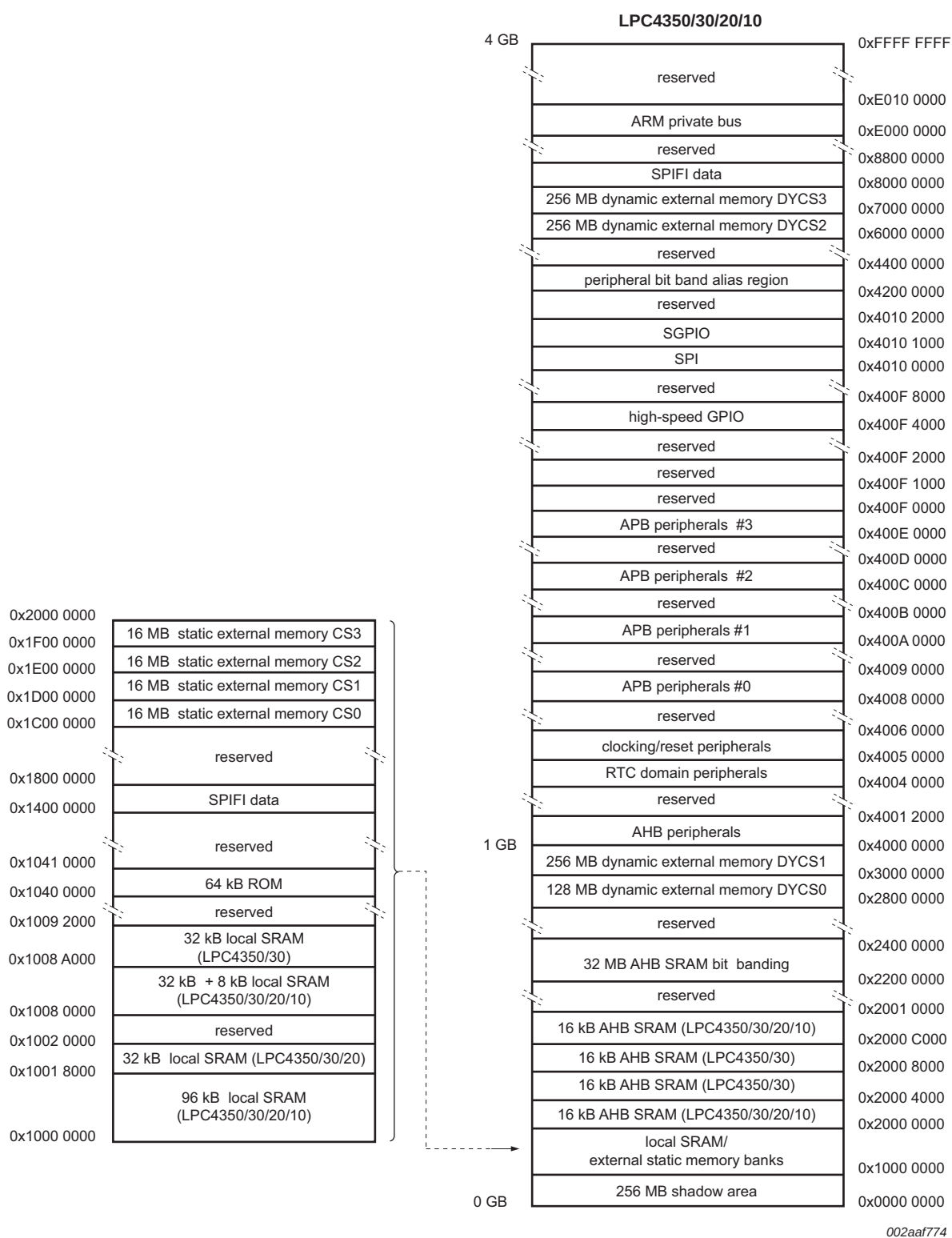
Fig 8. LPC4350/30/20/10 Memory mapping (overview)
