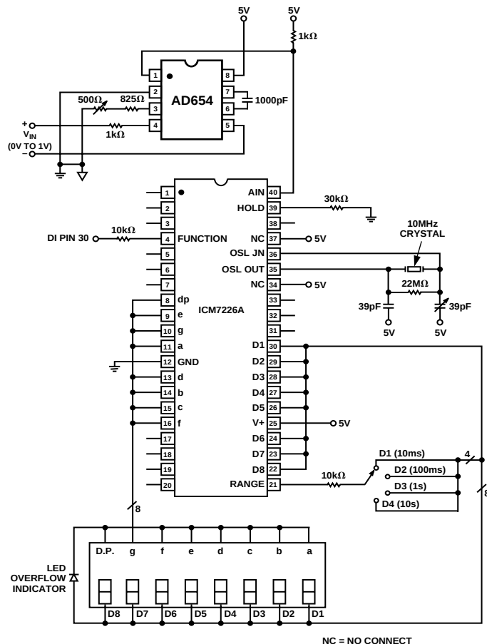
Figure 10. AD654 With Stand-Alone Frequency Counter/ LED Display Driver
