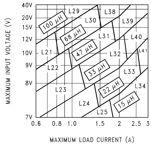
Figure 22. LM2596-5.0
