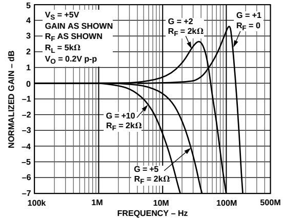
Figure 6. AD8054 Normalized Gain vs. Frequency; V_S = +5V
