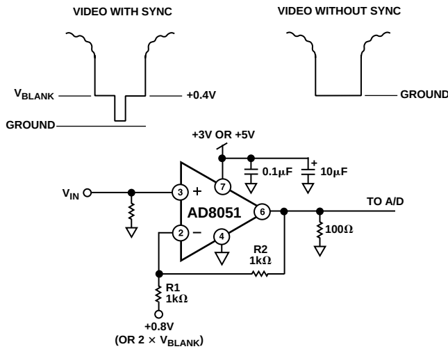
Figure 47. Sync Stripper
