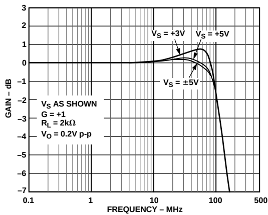
Figure 4. AD8051/AD8052 Gain vs. Frequency vs. Supply
