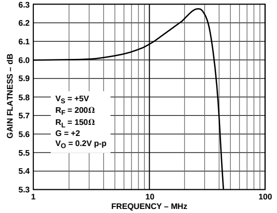
Figure 12. AD8054 0.1 dB Gain Flatness vs. Frequency; G = +2
