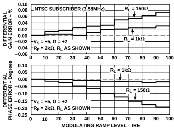
Figure 17. AD8051/AD8052 Differential Gain and Phase Errors
