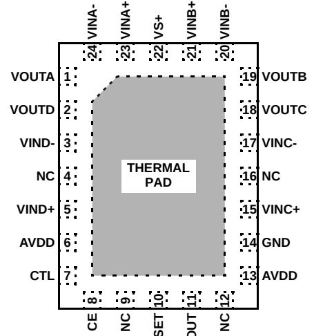
EL9202 (24 LD QFN) TOP VIEW
