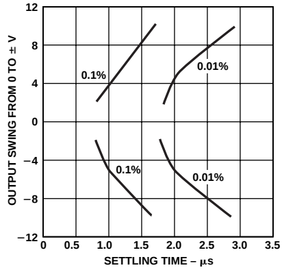
Figure 2. Settling Time
