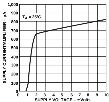
Figure 8. Supply Current vs. Supply Voltage
