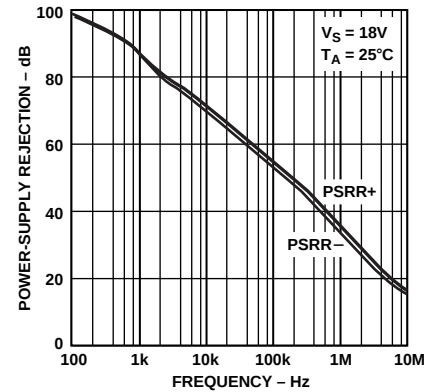
Figure 18. Power-Supply Rejection vs. Frequency
