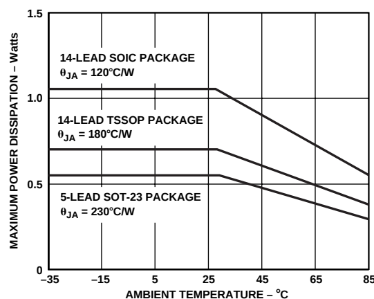
Figure 24. Maximum Power Dissipation vs. Temperature for 5-Lead and 14-Lead Package Types
