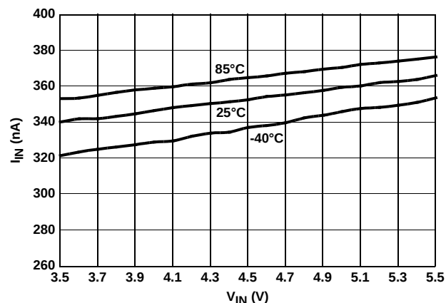
FIGURE 84. I_{IN} vs V_{IN} OVER TEMPERATURE
