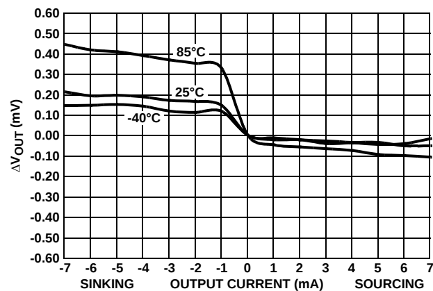
FIGURE 22. LOAD REGULATION
