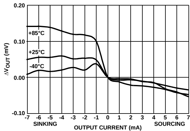
FIGURE 77. LOAD REGULATION
