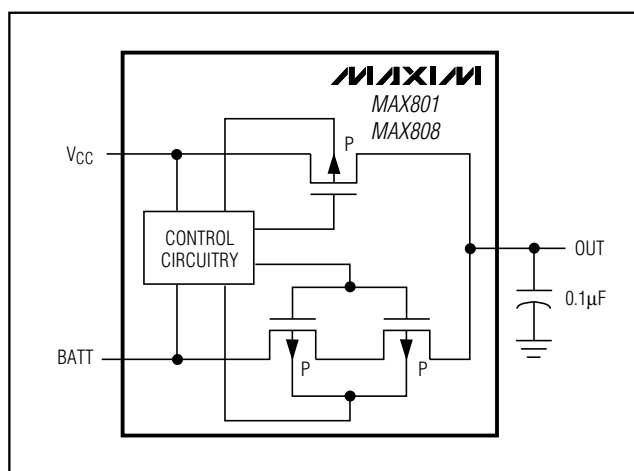
Figure 4. V_{CC} and BATT to OUT Switch
