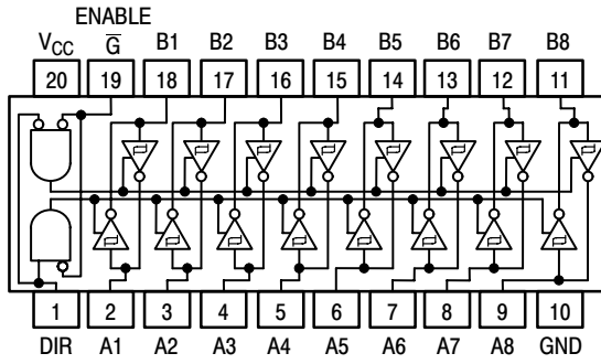
Figure 1. SN74LS640 SN74LS642
