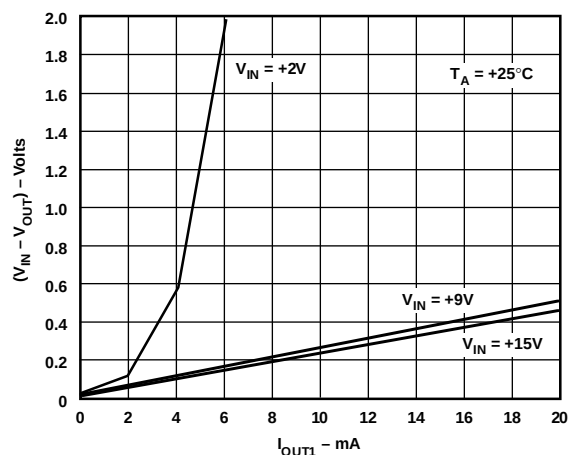
Figure 9. V_{OUT1} Input-Output Differential vs. Output Current
