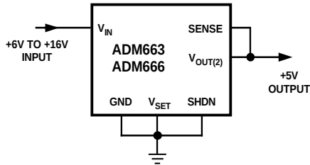
Figure 3. ADM663/ADM666 Fixed +5 V Output
