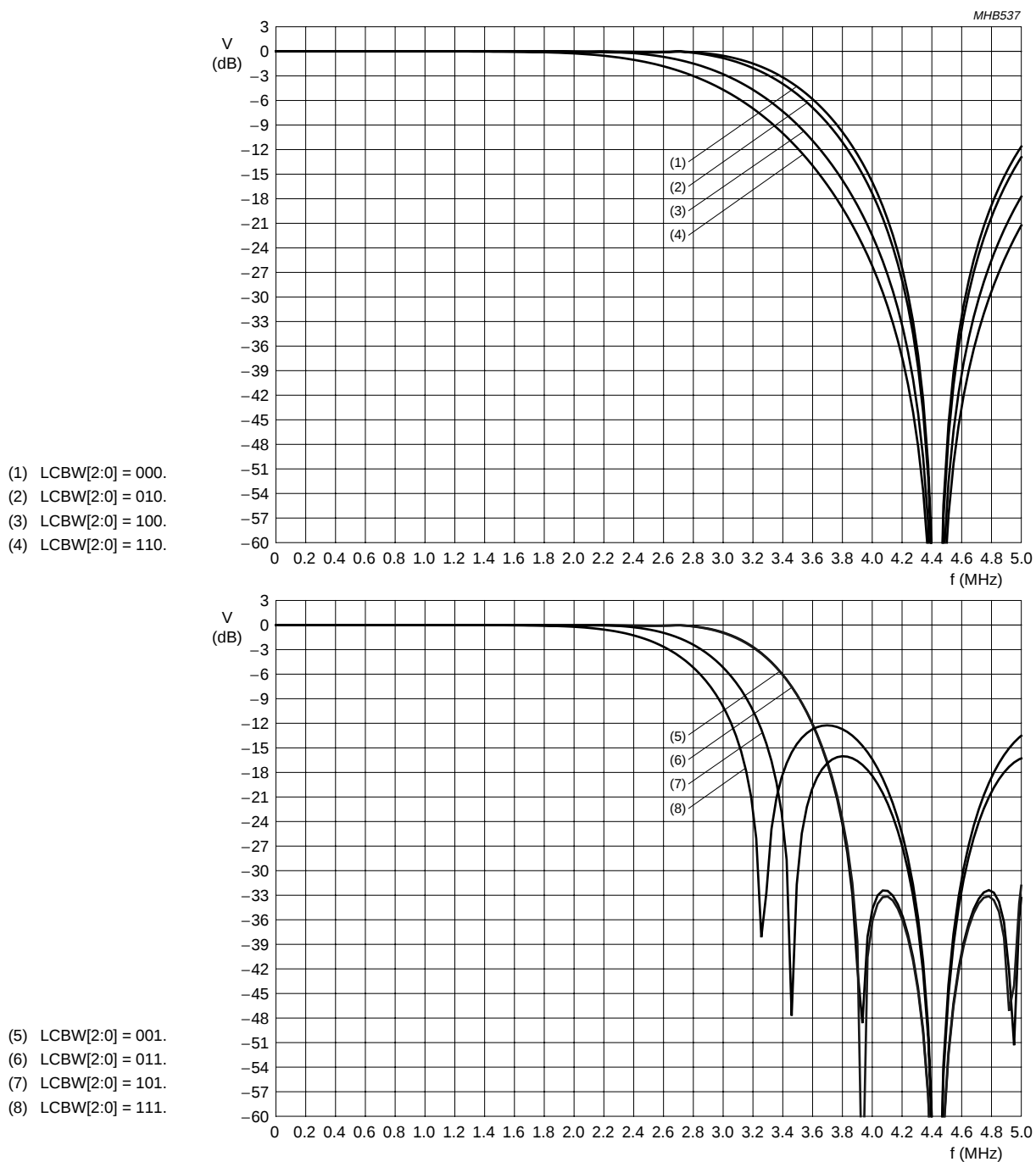
Fig.14 Transfer characteristics of the luminance notch filter in 4.43 MHz mode (Y-comb filter disabled) at LUBW = 0.
