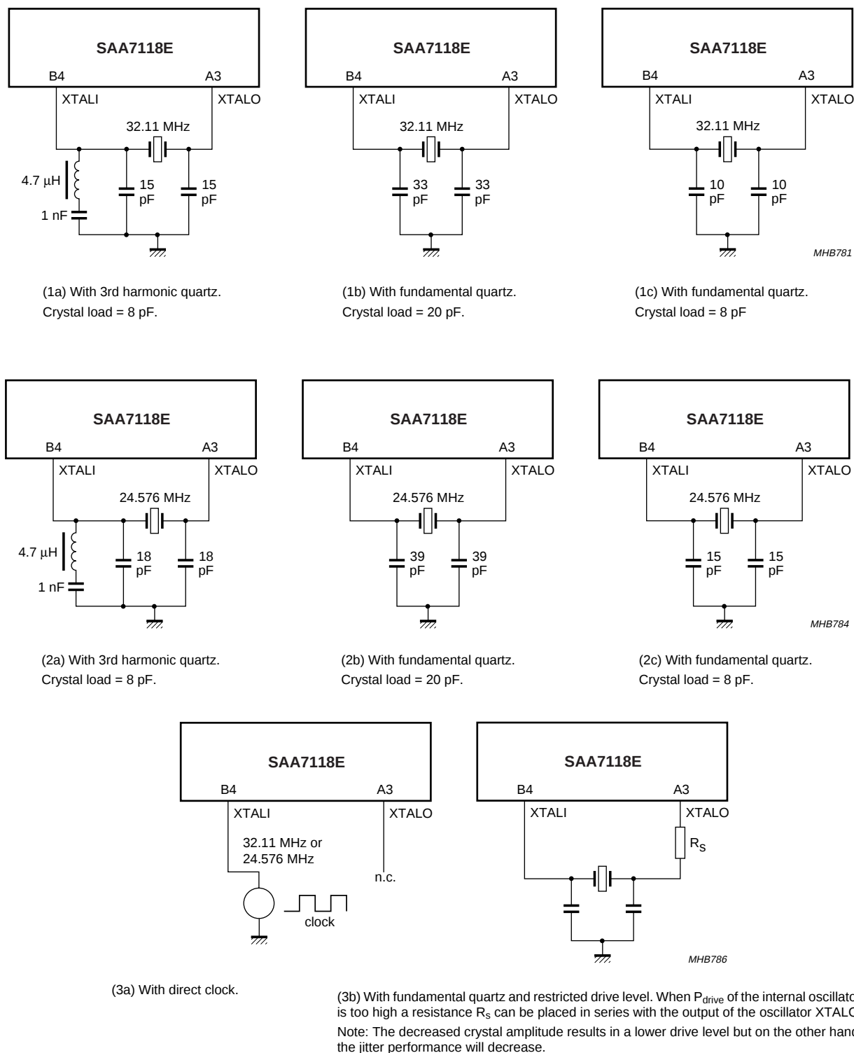
Fig.46 Oscillator application.
