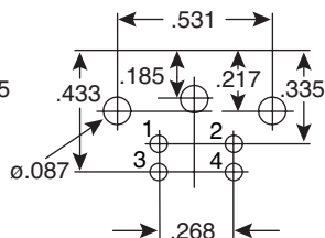
4-Pin 161-2304
