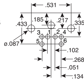
6-Pin 161-2306
