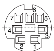
7-Pin 161-2307
