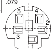
5-Pin 161-2305
