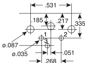
3-Pin 161-2303
