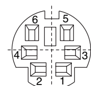
6-Pin 161-2306
