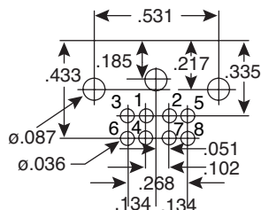
8-Pin 161-2308
