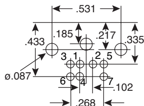
7-Pin 161-2307
