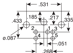
5-Pin 161-2305
