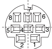
8-Pin 161-2308
