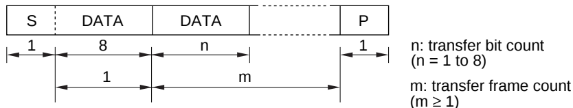
Figure 16.4 I²C Bus Data Format (Serial Format)
