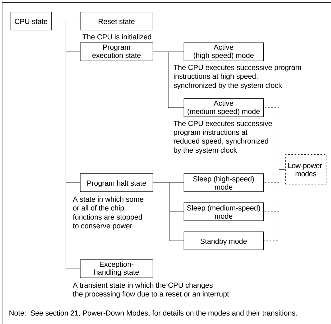
Figure 2.13 CPU Operation States
