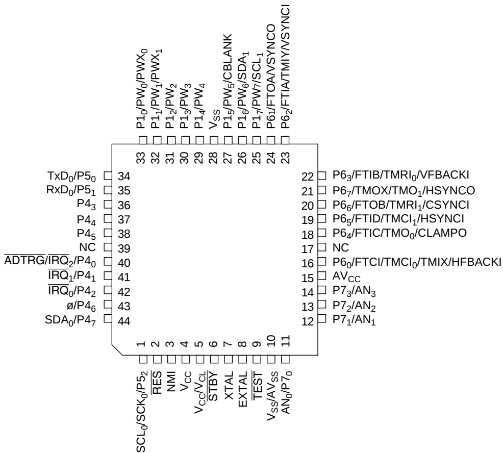
Figure 1.6 H8/3567 Series Pin Arrangement (No USB; FP-44A: Top View)
