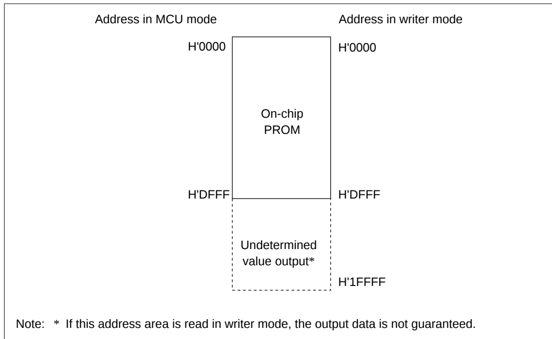
Figure 19.5 Memory Map in Writer Mode
