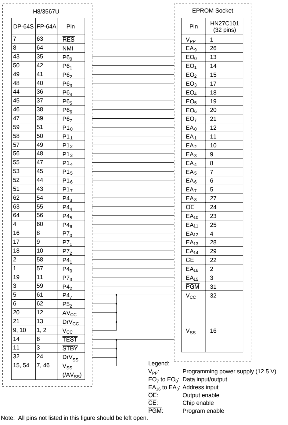
Figure 19.4 Socket Adapter Pin Assignments (H8/3567U)
