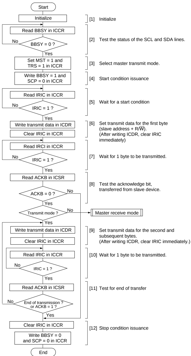
Figure 16.13 Flowchart for Master Transmit Mode (Example)
