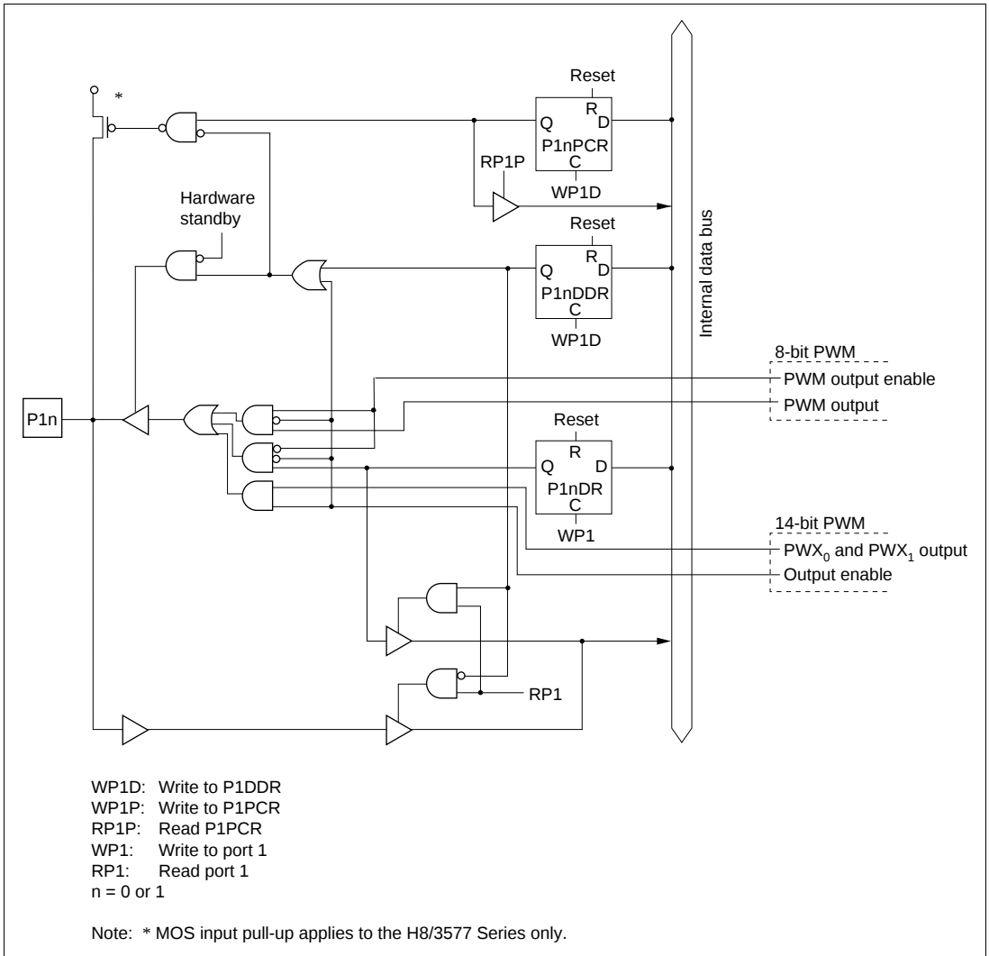
Figure C.1 Port 1 Block Diagram (Pins P1 0 and P1 1 )
