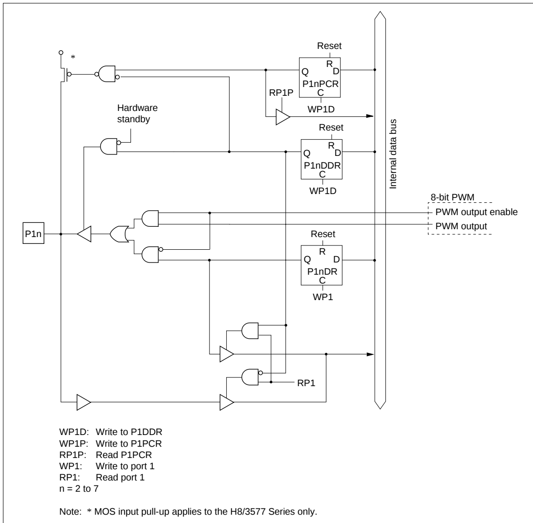
Figure C.2 Port 1 Block Diagram (Pins P1 2 to P1 7 in H8/3577 Series, Pins P1 2 to P1 4 in H8/3567 Series)
