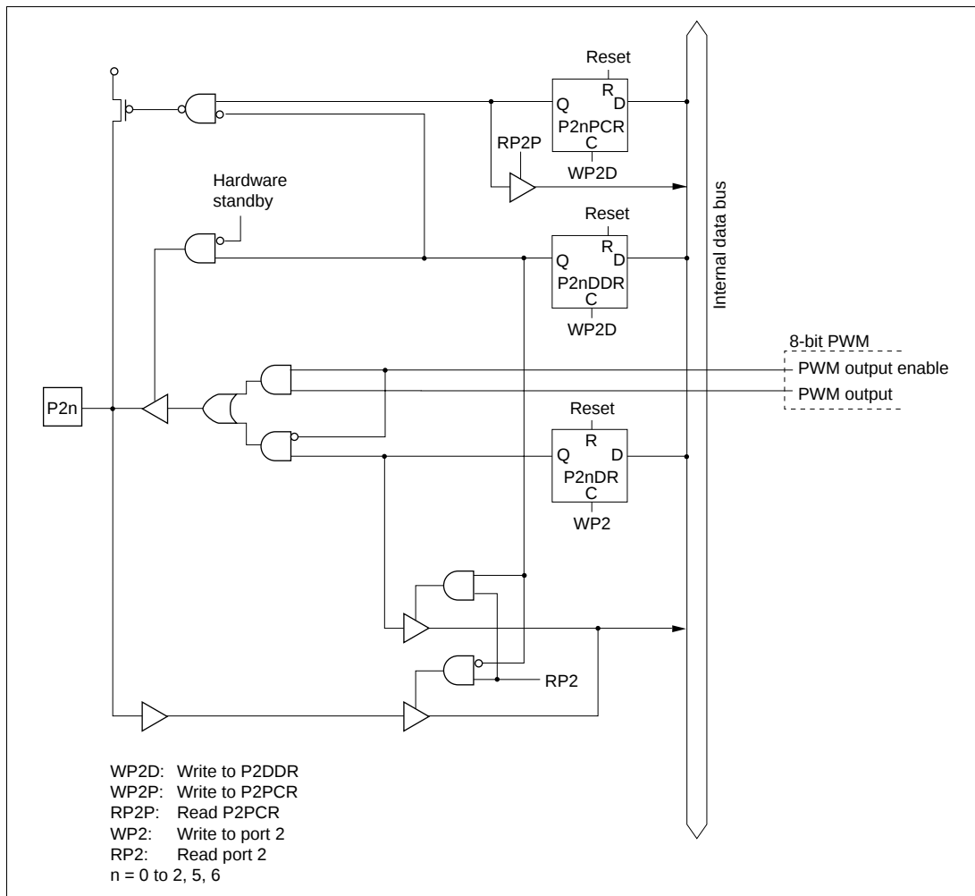
Figure C.6 Port 2 Block Diagram (Pins P2 0 to P2 2 , P2 5 , and P2 6 in H8/3577 Series)
