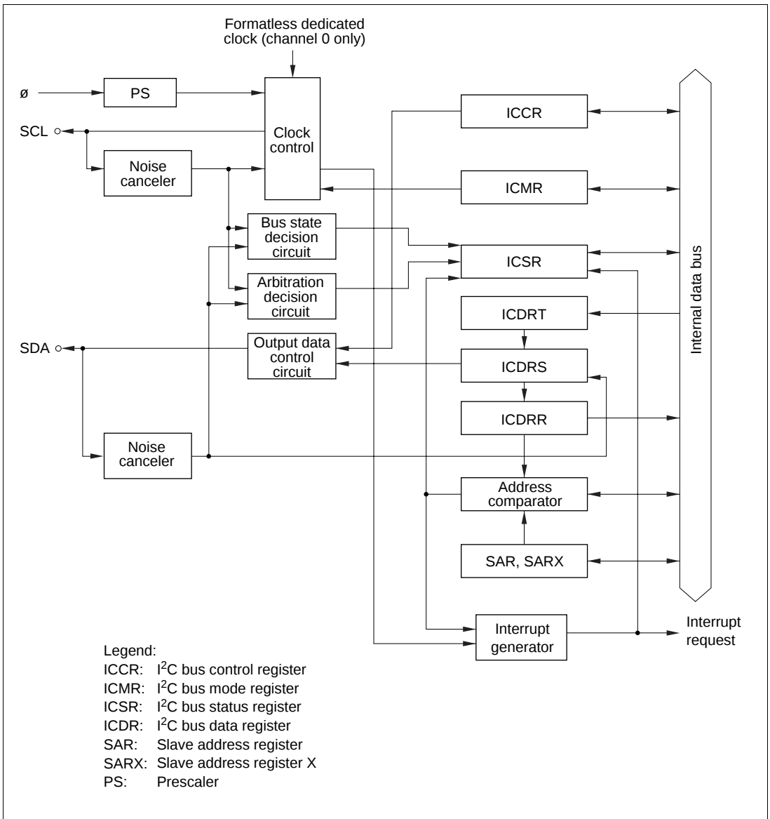
Figure 16.1 Block Diagram of I²C Bus Interface
