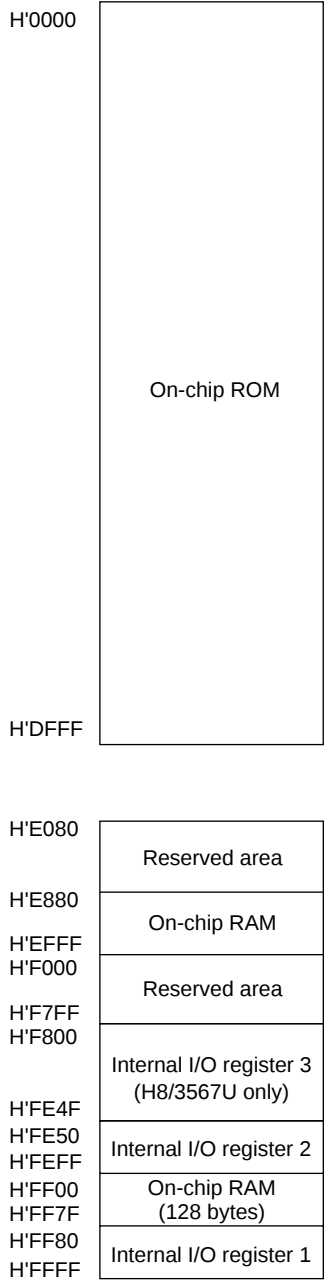
Figure 3.1 H8/3577, H8/3567, and H8/3567U Address Map
