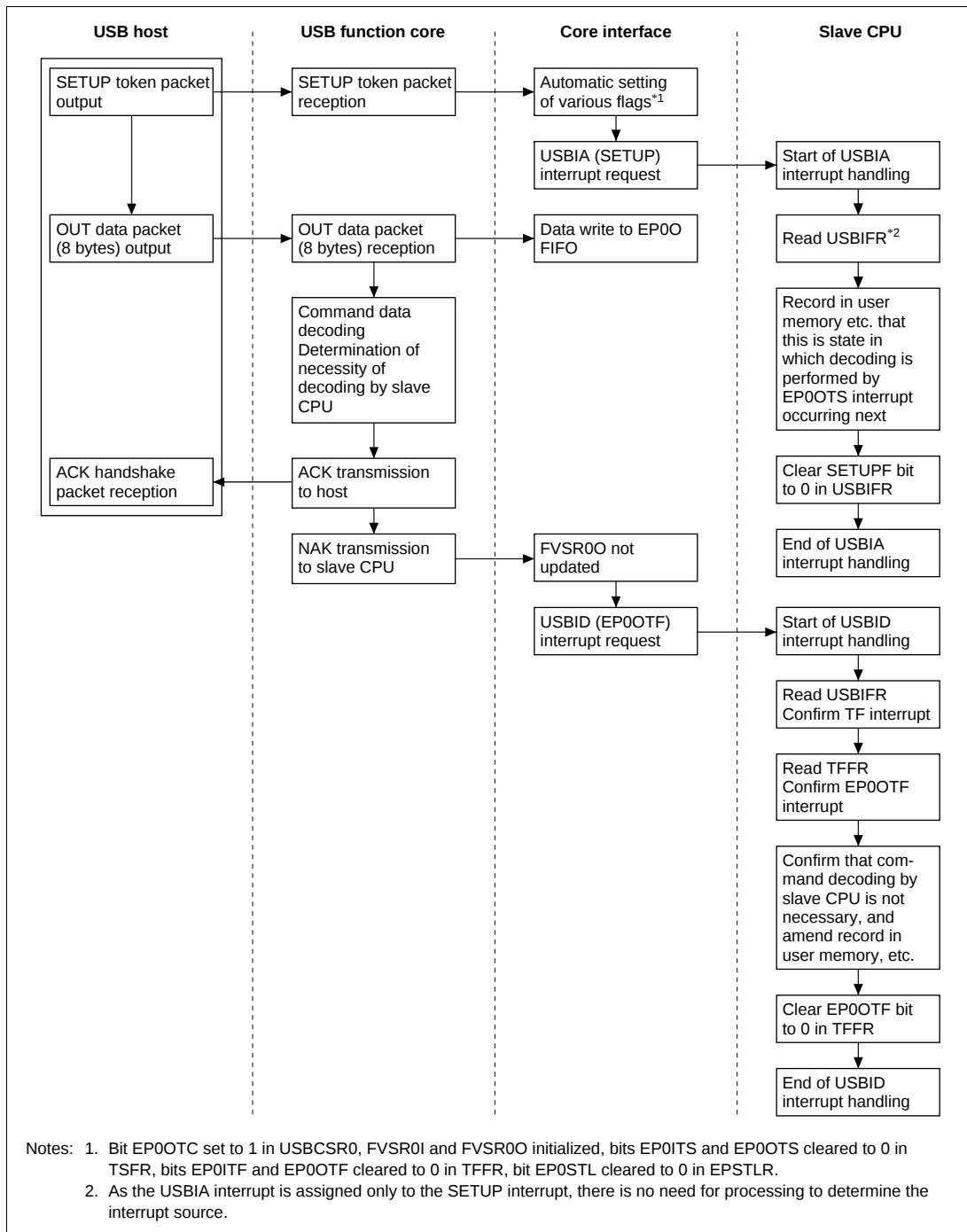
Figure 7.2 (1) Operation when SETUP Token is Received (Decoding by Slave CPU Not Required)
