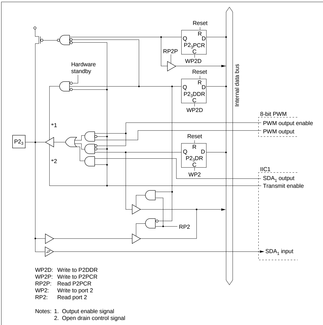
Figure C.7 Port 2 Block Diagram (Pin P2 3 in H8/3577 Series)
