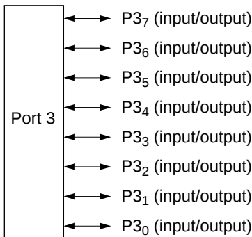
Figure 8.3 Port 3 Pin Functions
