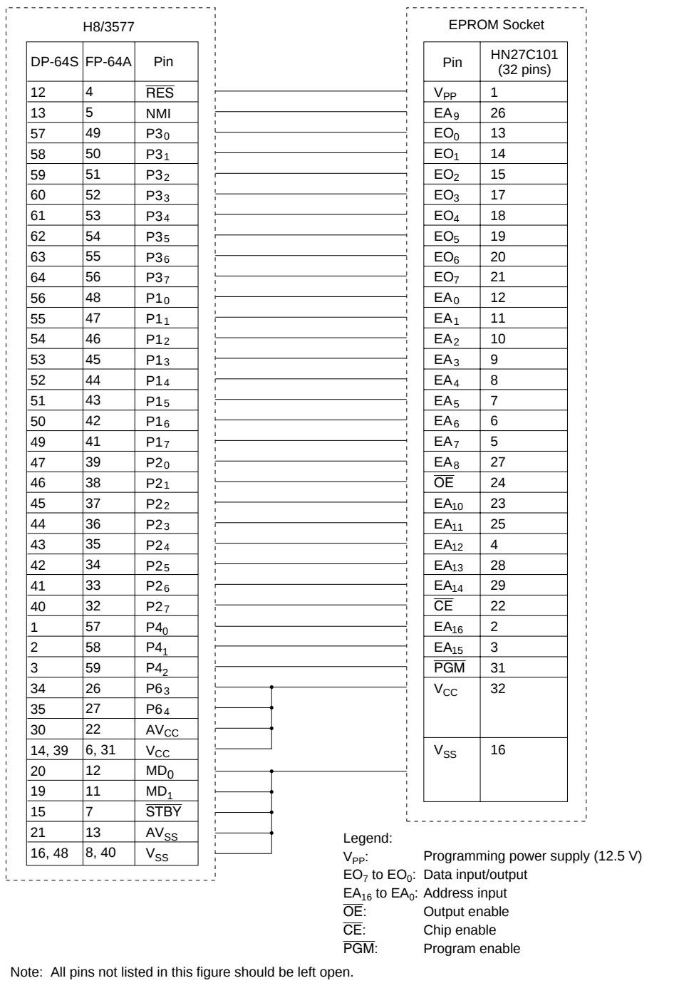
Figure 19.2 Socket Adapter Pin Assignments (H8/3577)
