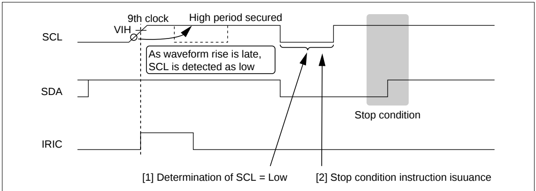
Figure 16.19 Timing of Stop Condition Issuance
