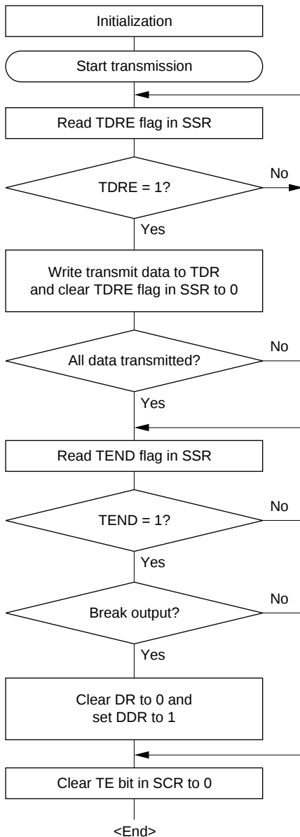
Figure 15.5 Sample Serial Transmission Flowchart
