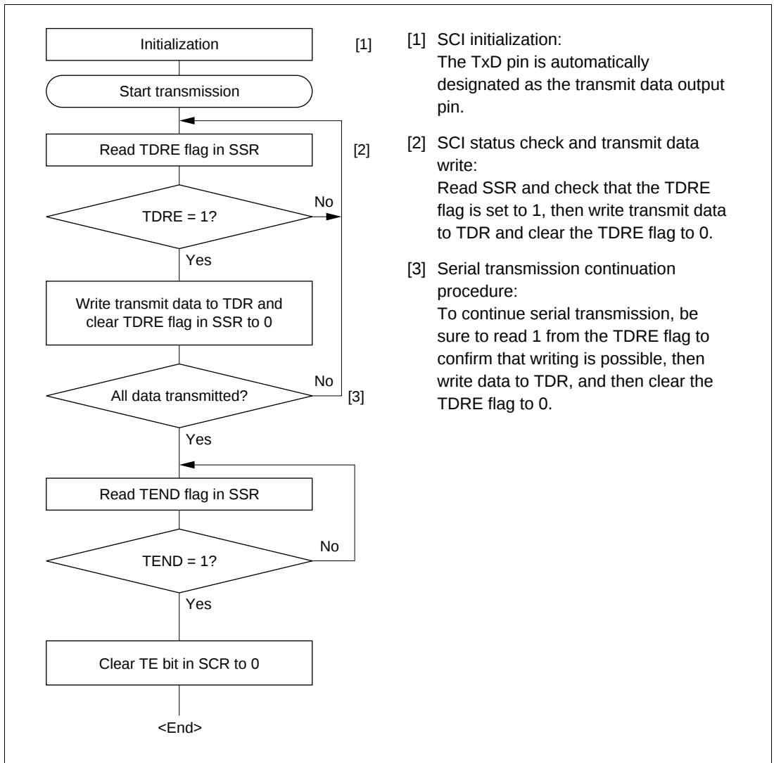
Figure 15.16 Sample Serial Transmission Flowchart
