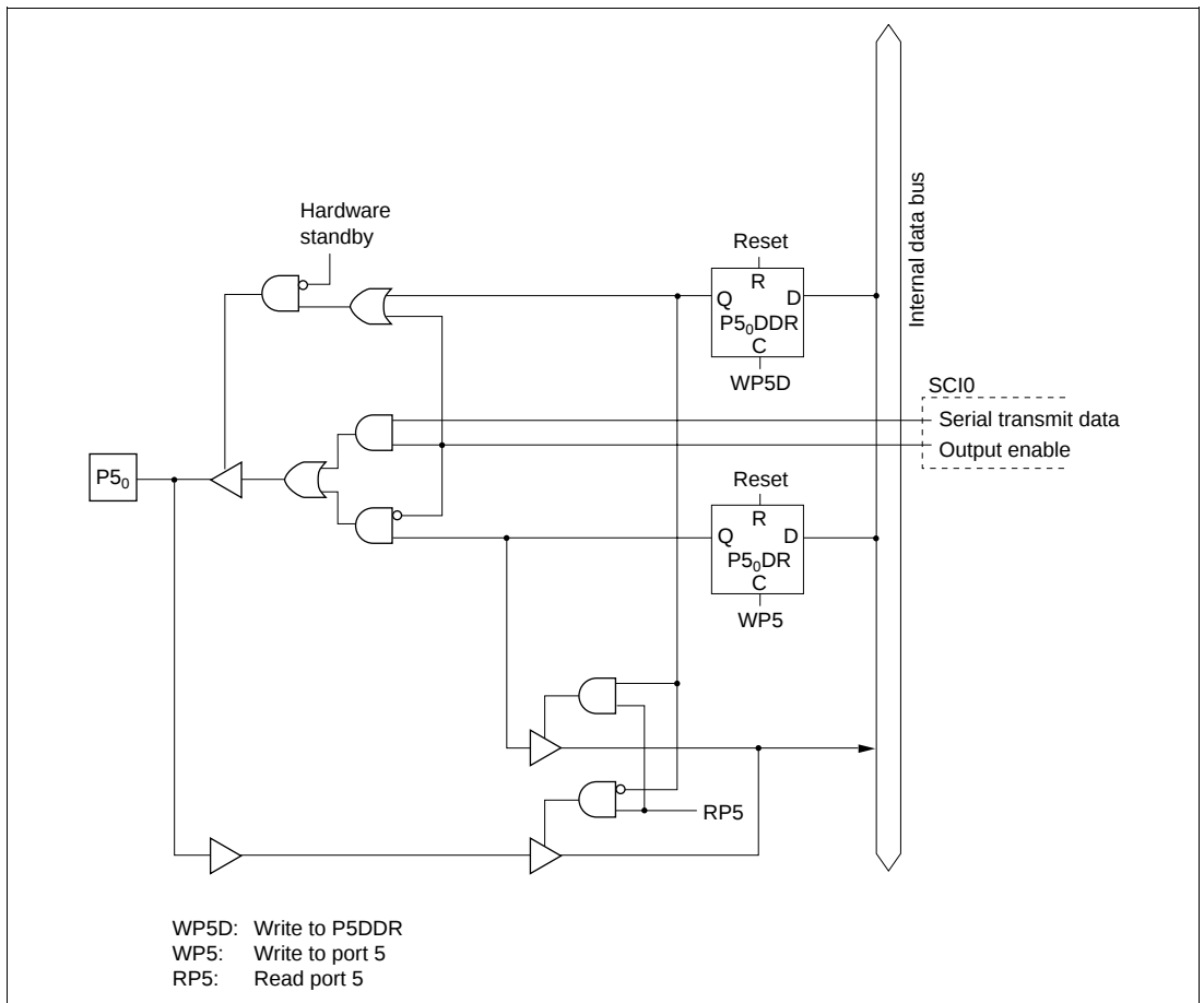
Figure C.16 Port 5 Block Diagram (Pin P5 0 )
