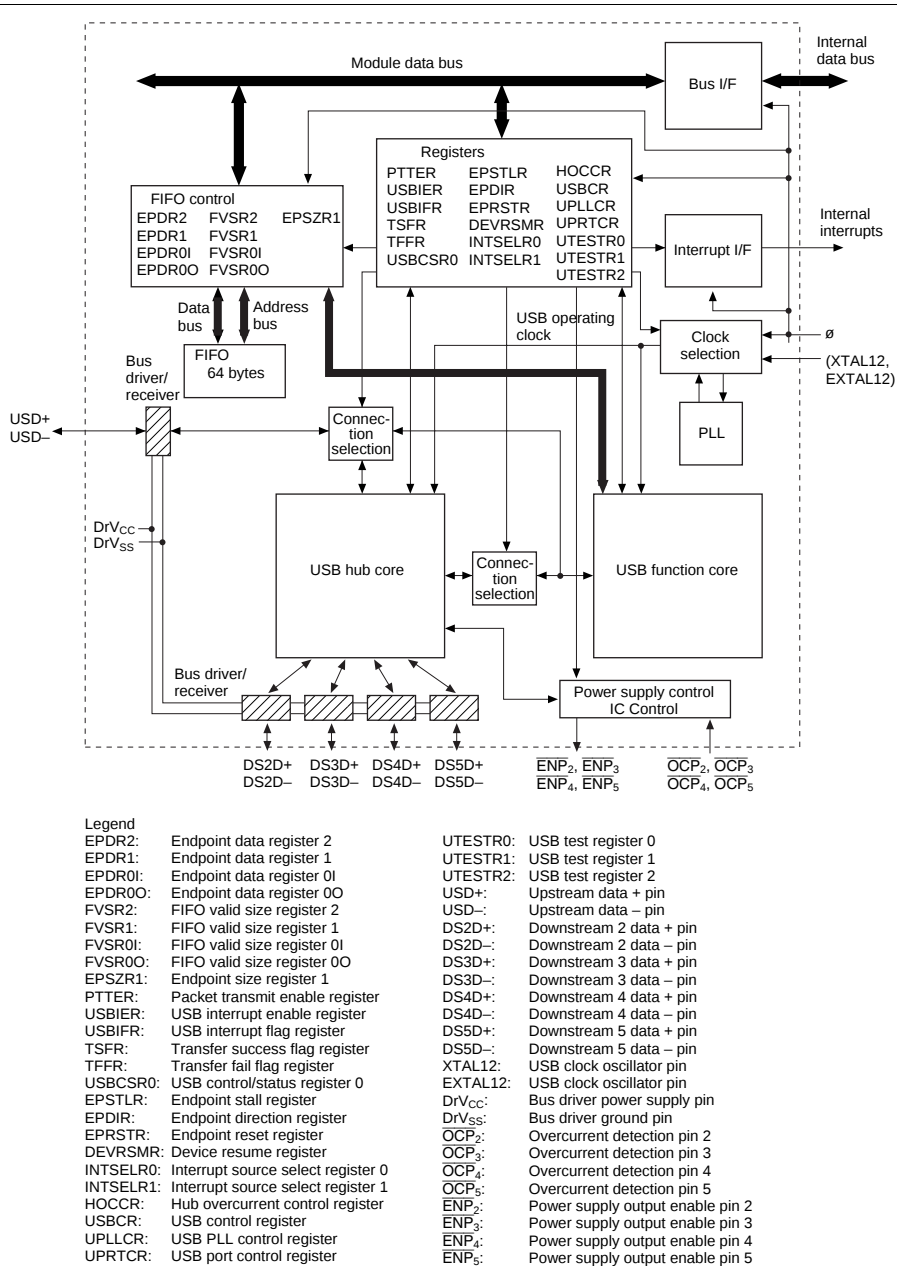
Figure 7.1 Block Diagram of USB
