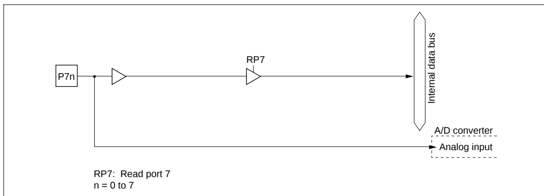
Figure C.24 Port 7 Block Diagram (Pins P7 0 to P7 7 in H8/3577 Series, Pins P7 0 to P7 3 in H8/3567 Series)
