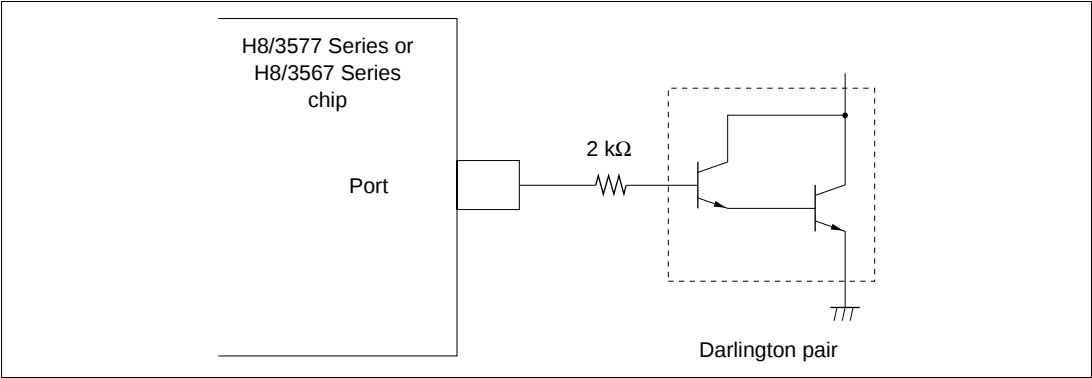
Figure 22.1 Darlington Pair Drive Circuit (Example)
