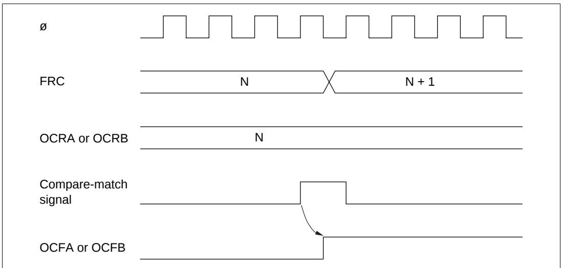
Figure 11.12 Setting of Output Compare Flag (OCFA, OCFB)
