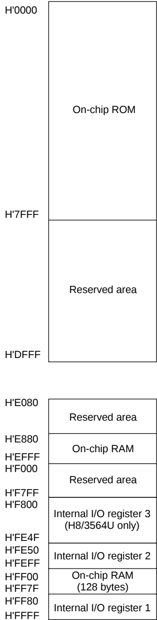
Figure 3.2 H8/3574, H8/3564, and H8/3564U Address Map
