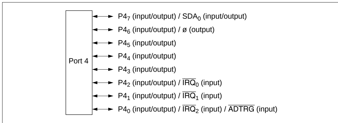
Figure 8.4 Port 4 Pin Functions
