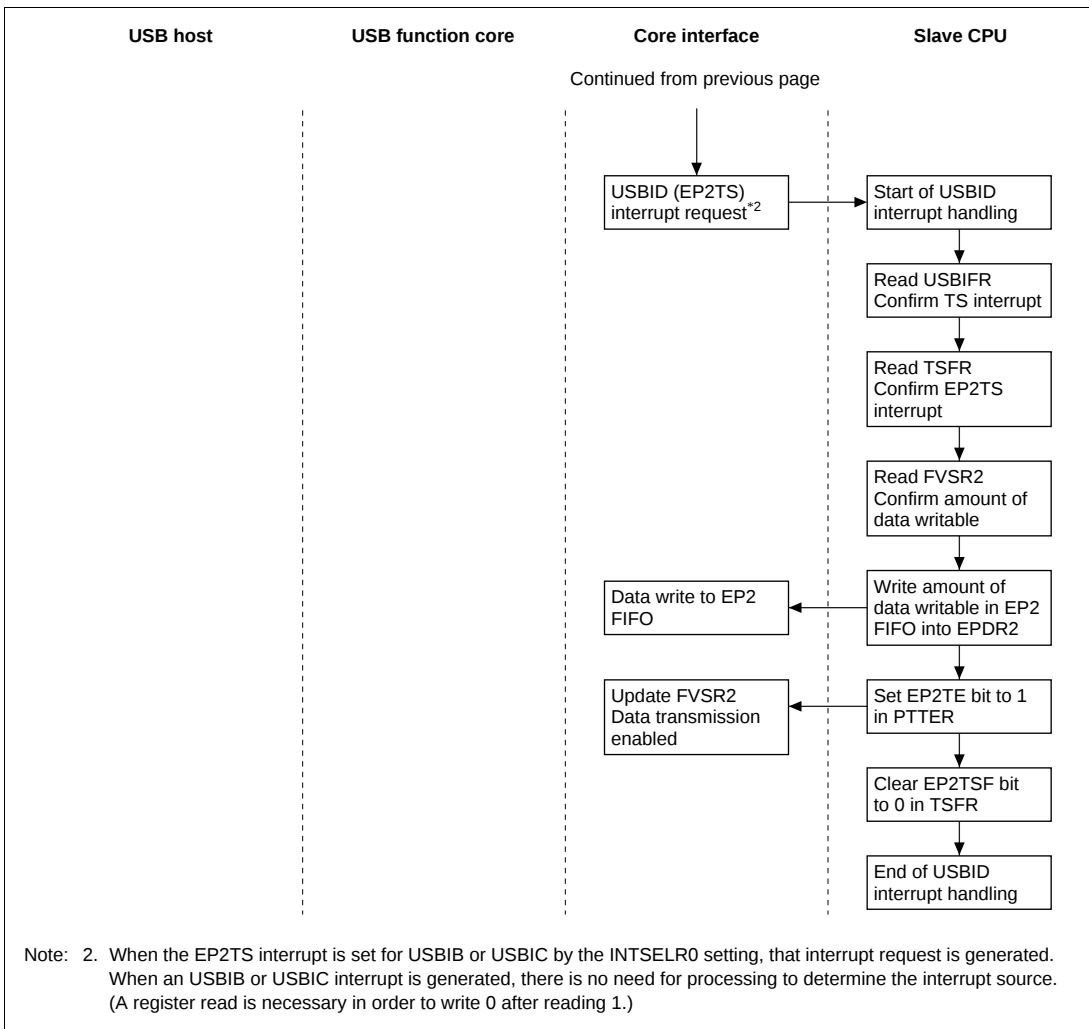
Figure 7.4 (1) Operation when IN Token is Received (EP2-IN: Initial FIFO Empty) (cont)
