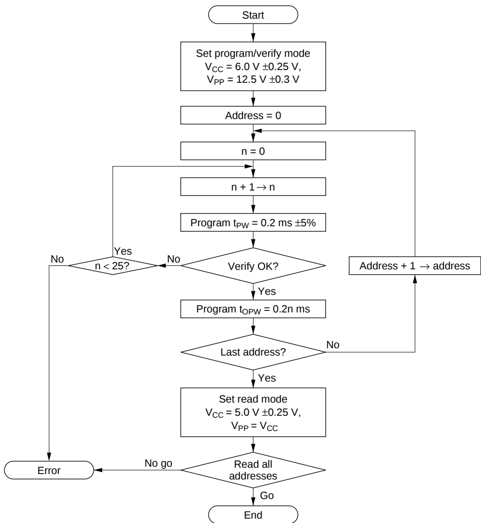
Figure 19.6 High-Speed Programming Flowchart
