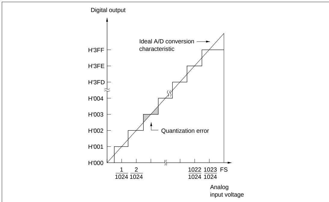
Figure 17.9 A/D Conversion Precision Definitions (1)
