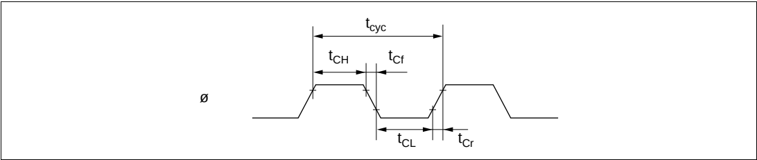
Figure 22.3 System Clock Timing
