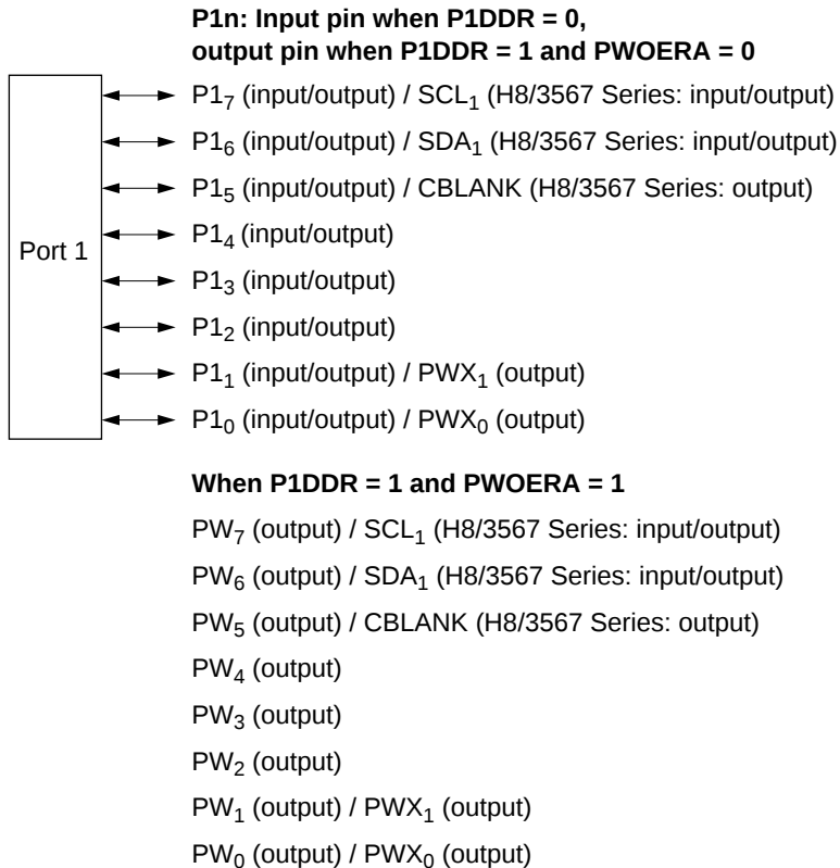
Figure 8.1 Port 1 Pin Functions
