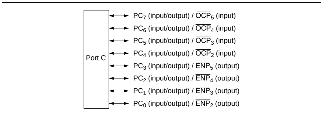
Figure 8.8 Port C Pin Functions
