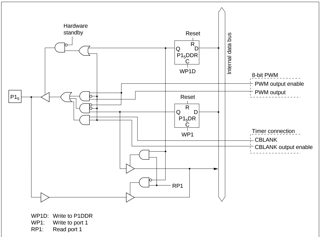
Figure C.3 Port 1 Block Diagram (Pin P1 5 in H8/3567 Series)
