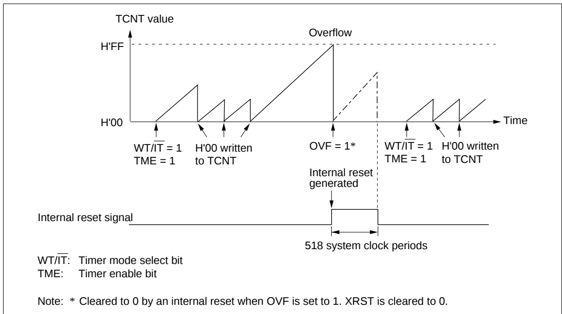
Figure 14.3 Operation in Watchdog Timer Mode
