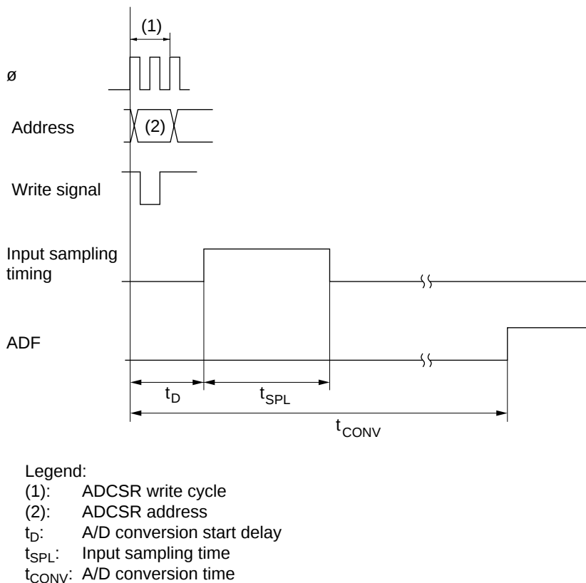
Figure 17.5 A/D Conversion Timing
