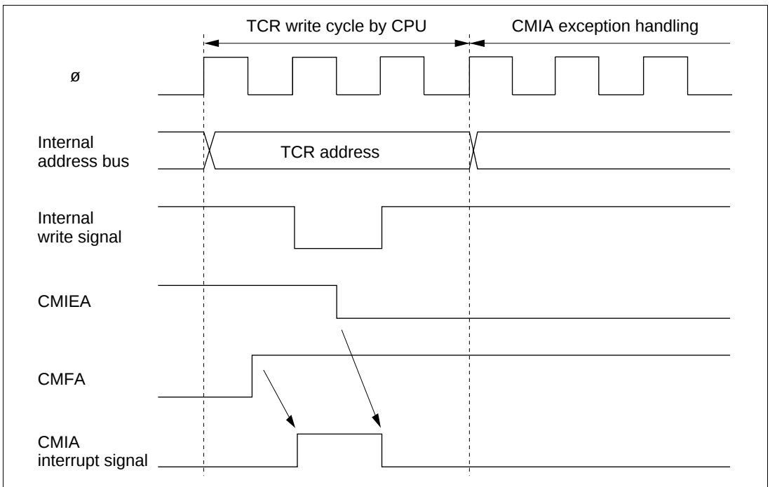
Figure 5.7 Contention between Interrupt Generation and Disabling
