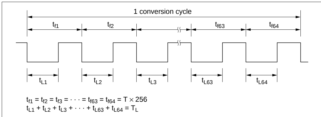
Figure 10.4 (2) Output Waveform
