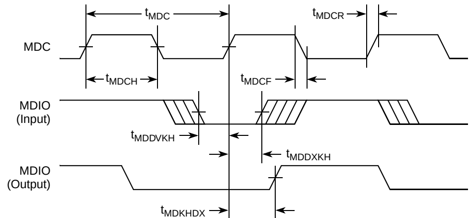
Figure 17. MII Management Interface Timing Diagram
