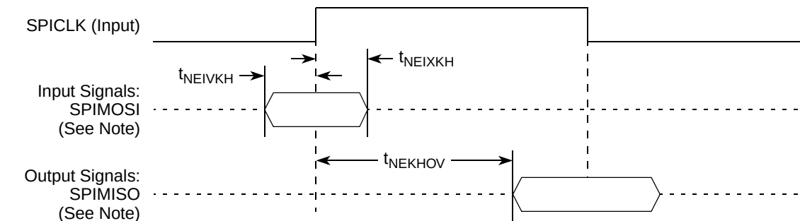
Figure 57. SPI AC Timing in Slave Mode (External Clock) Diagram
