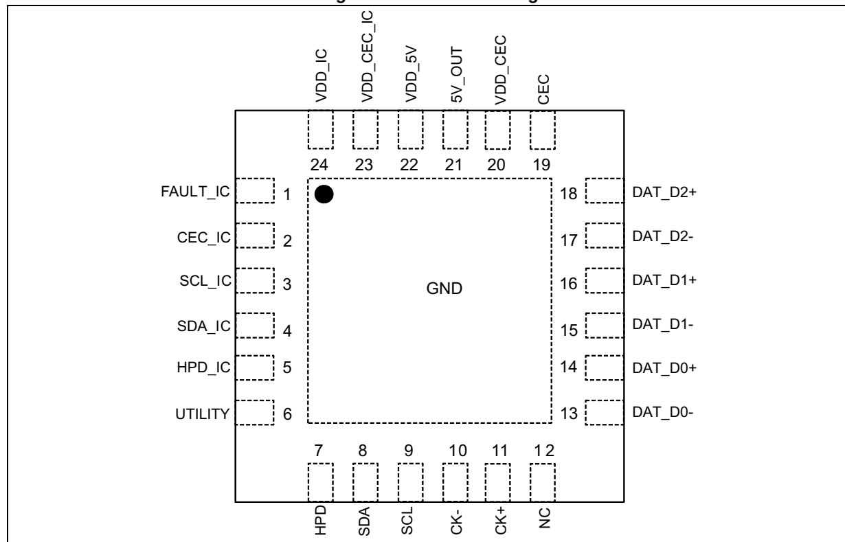
Figure 12. Pin numbering
