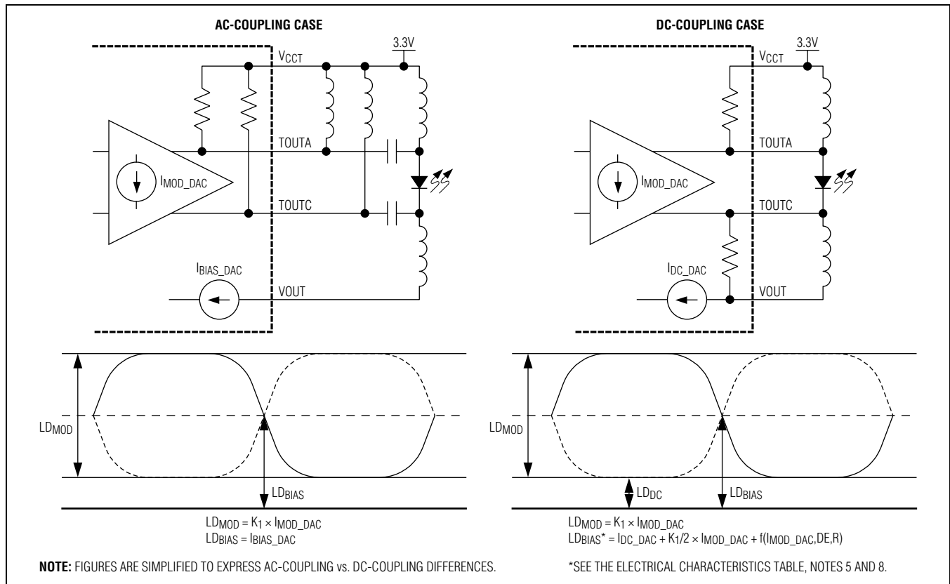
Figure 3. AC-/DC-Coupling Cases
