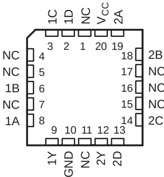
54AC11020 . . . FK PACKAGE (TOP VIEW)
