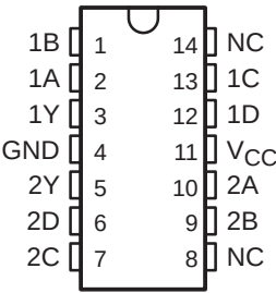
54AC11020 . . . J PACKAGE 74AC11020 . . . D OR N PACKAGE (TOP VIEW)
