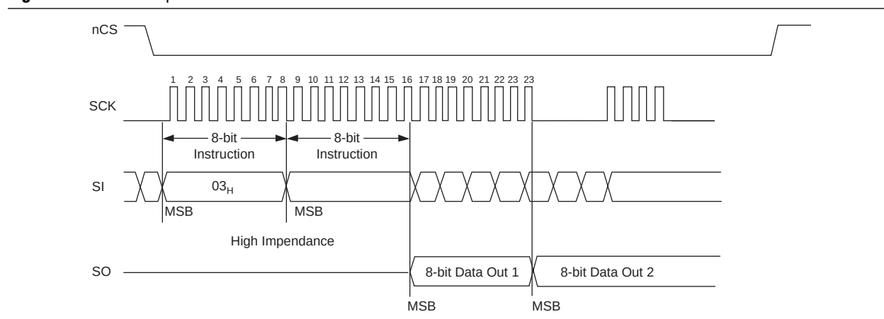
Figure 9-27. READ Operation for Base Mode
