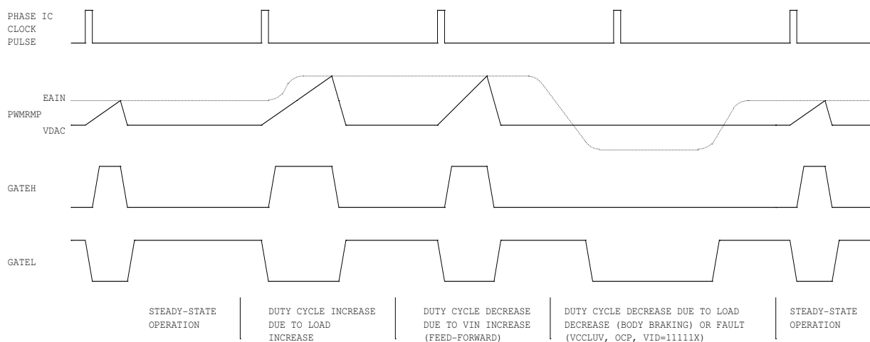
Figure 3 PWM Operating Waveforms
