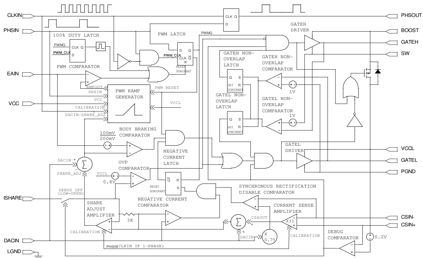
Figure 5 Block diagram
