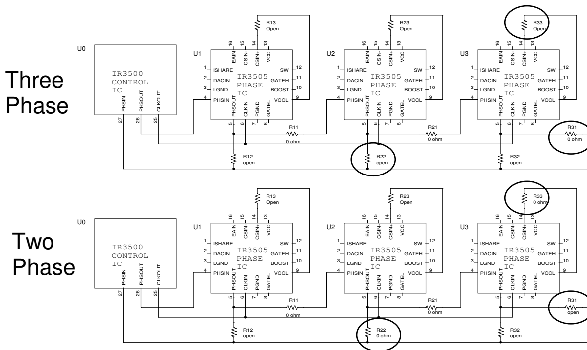
Figure 7 – Optional Phase application circuit
