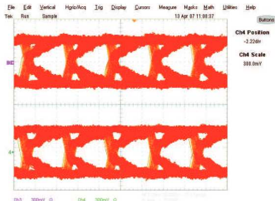
Tx buffers only running at 400 Mbps; Channel 3: 1Y-1Z, Channel 4: 2Y-2Z
