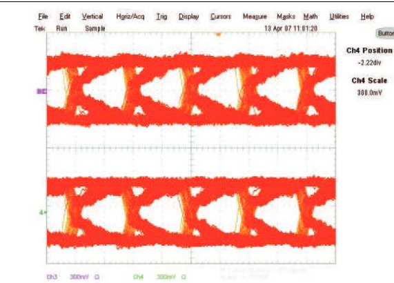
Tx buffers only running at 400 Mbps; Channel 3: 1Y-1Z, Channel 4: 2Y-2Z
