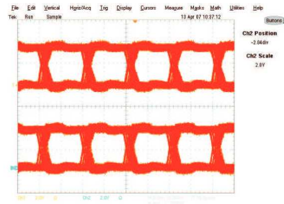
Rx buffers only running at 100 Mbps; Channel 1: R, Channel 2: 2R
