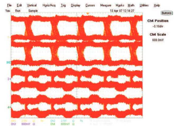
All buffers running at 100 Mbps; Channel 1: R, Channel 2: 2R, Channel 3: 1Y-1Z, Channel 4: 2Y-2Z
