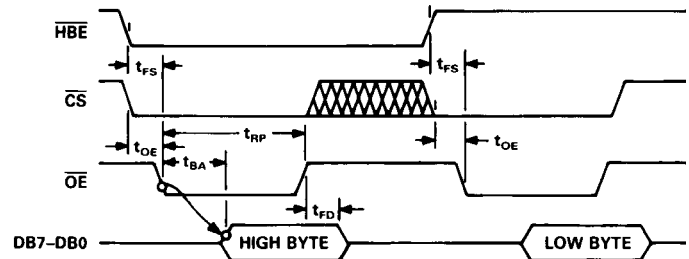
Figure 2. Output Timing
