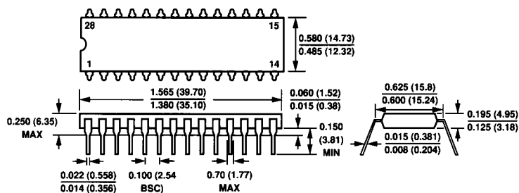
28-Lead Plastic DIP Package (N-28)
