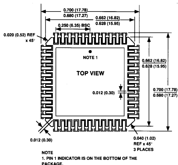
44-Lead J-Leaded Chip Carrier (J-44)
