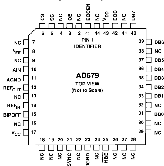
JLCC Package
