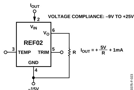
Figure 24. Current Sink
