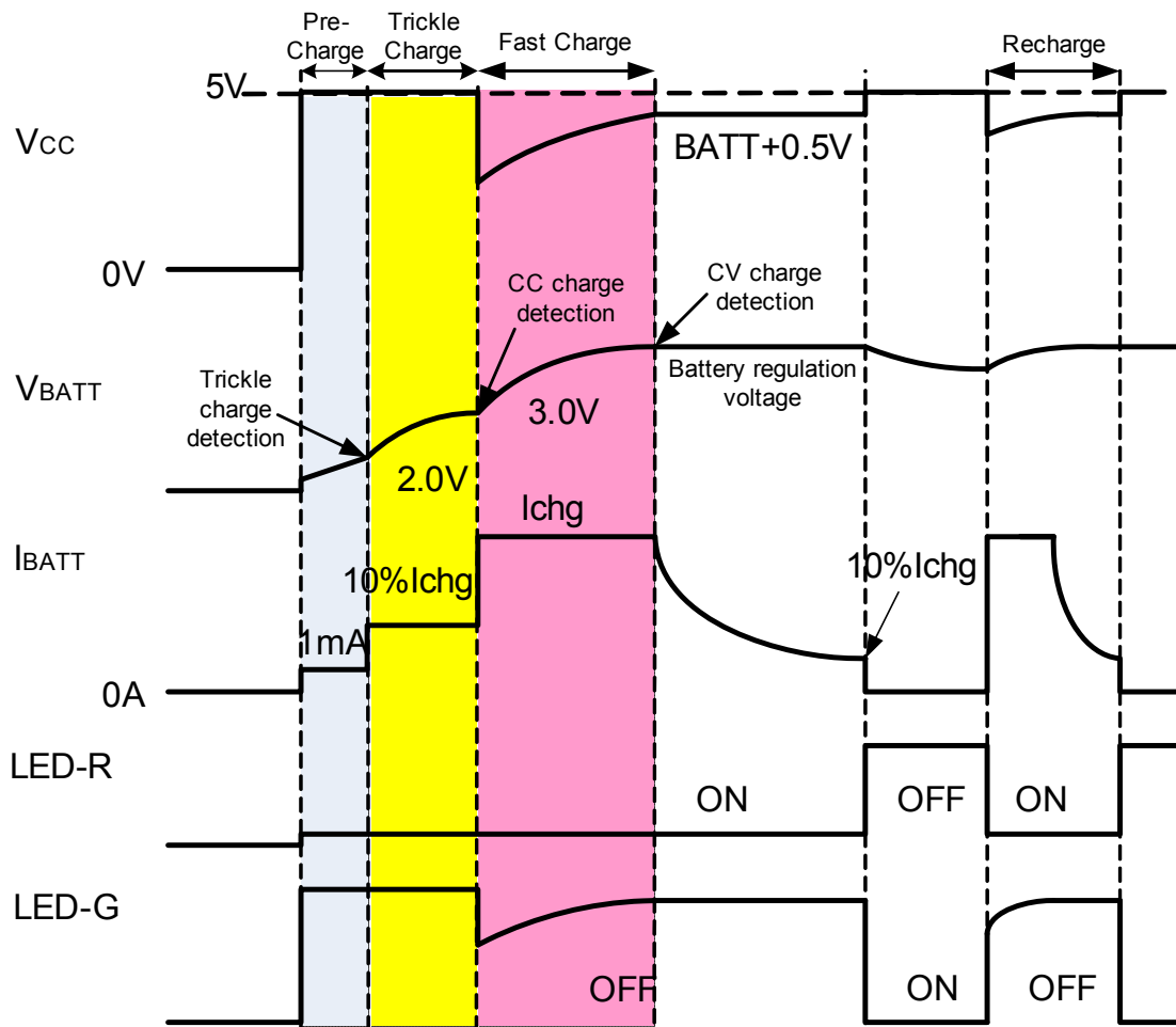
Figure 3— Typical Charge Profile
