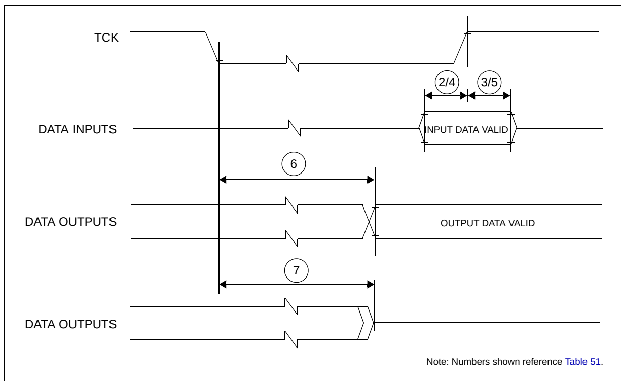
Figure 35. Timing diagram - JTAG boundary scan
