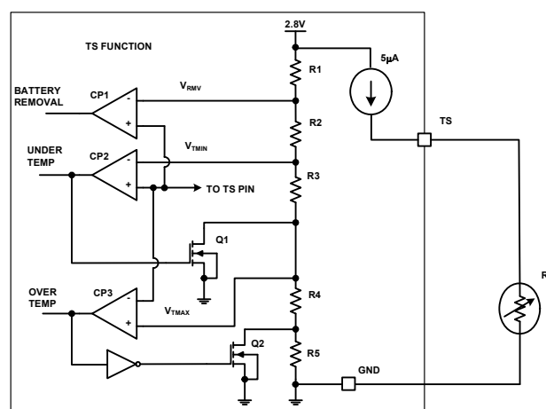
FIGURE 2. INTERNAL CIRCUIT FOR NTC INTERFACE
