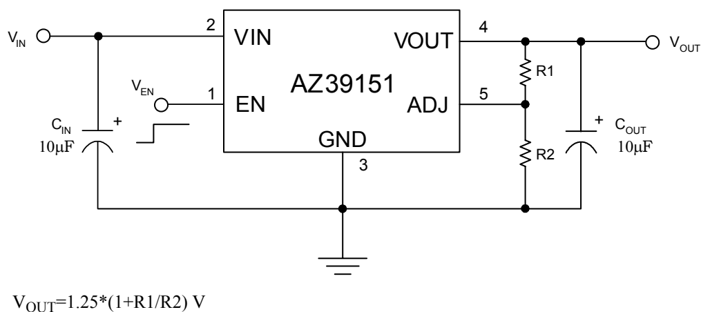
Adjustable Version
