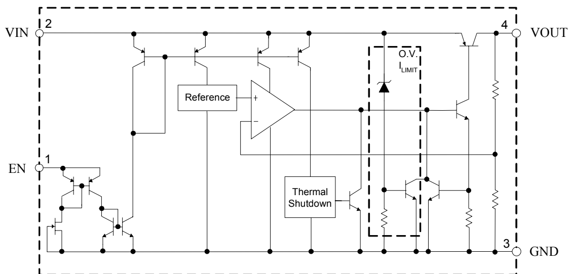
Fixed Version
