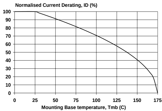
Fig.2. Normalised continuous drain current. ID\% = 100 \cdot I_D / I_{D\ 25\ ^\circ\text{C}} = f(T_{mb}) ; V_{GS} \geq 10\text{ V}
