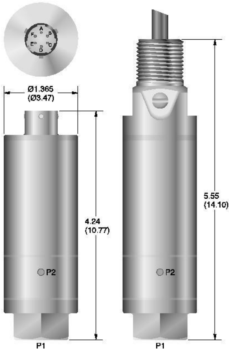
Figure 9.3—PPTR Case Outline
