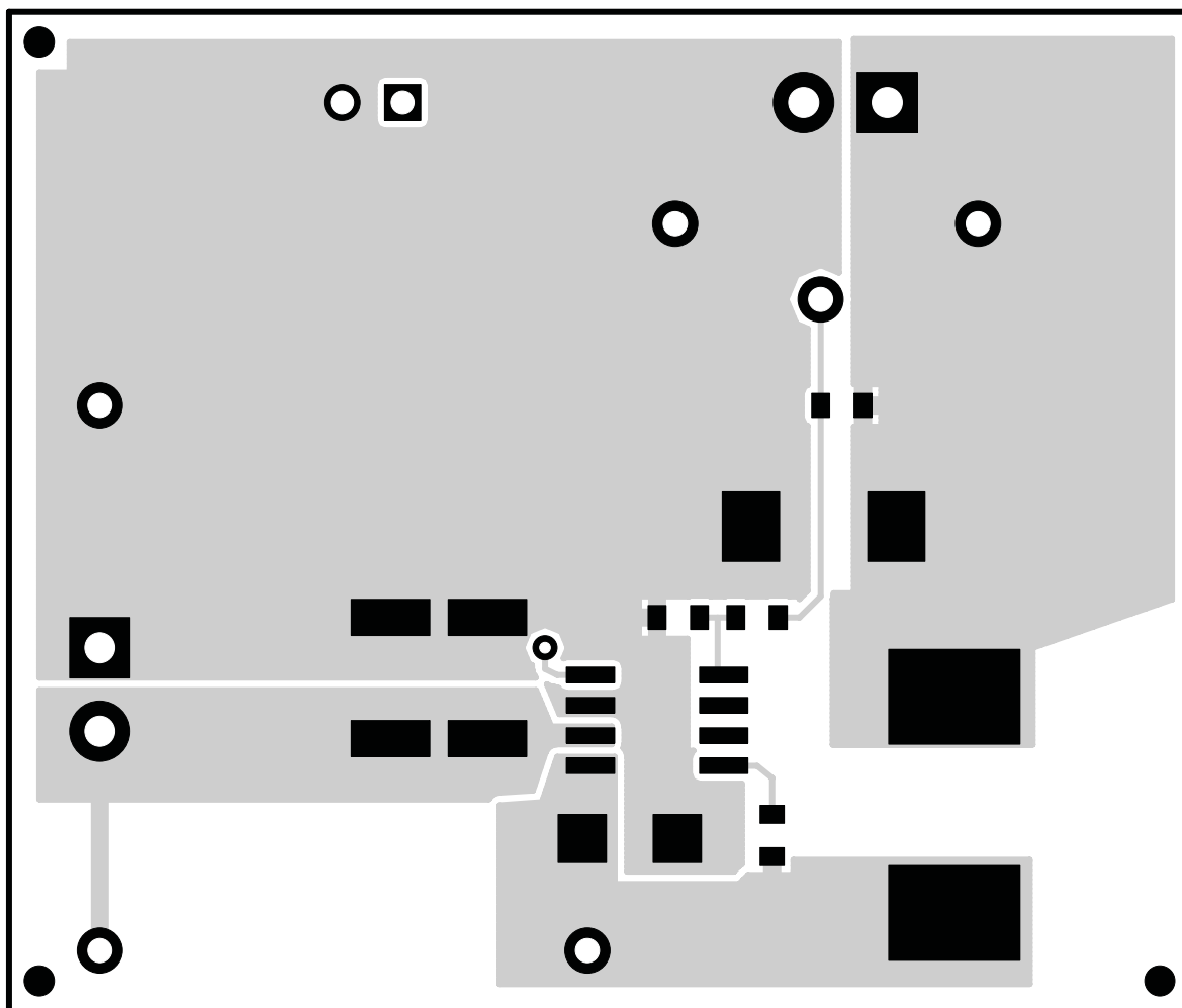
Figure 10. Top-Side Layout
