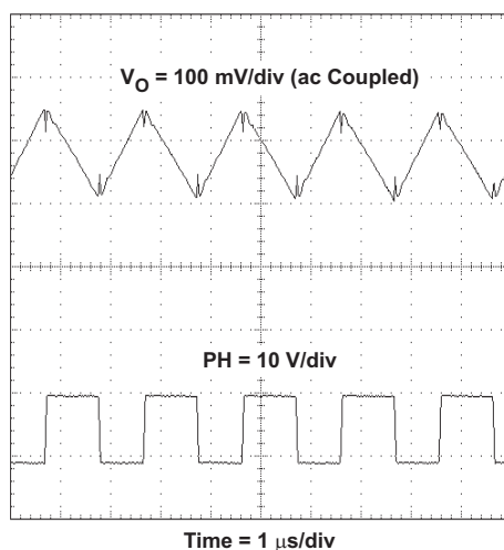
Figure 7. Input Voltage Ripple, TPS5420
