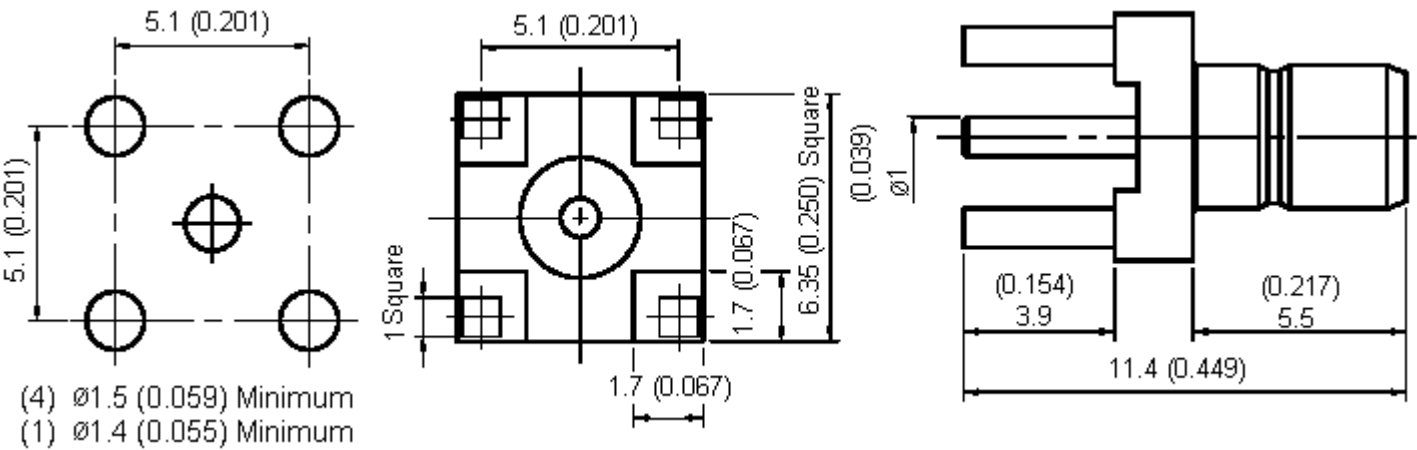
Mounting Hole
