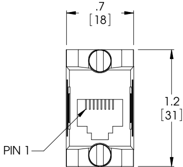
"J1" RJ45 JACK (8X8)
