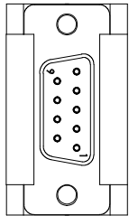
"P1" 9 CONTACT FEMALE D-SUB CONNECTOR
