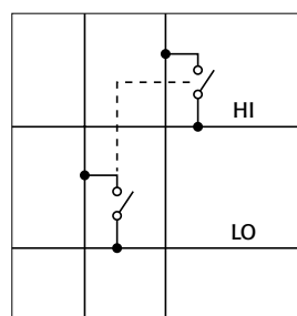
Matrix Crosspoint
