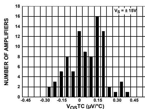
FIGURE 2. V_{OS} TEMPERATURE COEFFICIENT ( V_{OS} TC )
